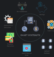
Smart Contracts
